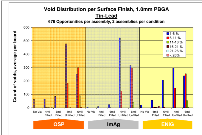
Figure 22. Voiding occurrence in 1.0mm PBGA with no vias, 4-mil vias, and 6-mil vias. Again, the Y-axis scale has changed due to higher opportunity count. In this case, the ENIG finish appears to produce less voids than OSP or ImAg.
