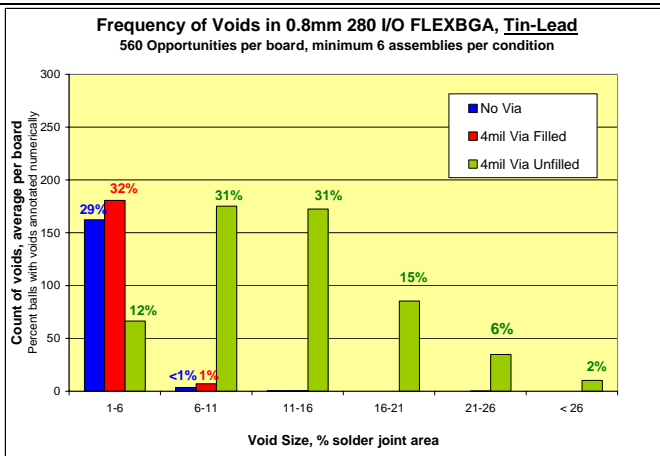
Figure 12. Frequency of Voids in 0.8mm 280 I/O BGA with tin-lead alloy. Notice change in Y-axis scale from previous
