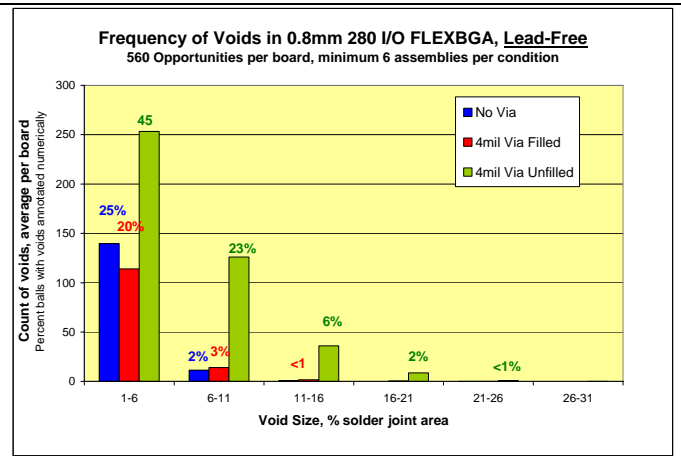
Figure 13. Frequency of Voids in 0.8mm 280 I/O BGA with lead-free alloy. Notice change in Y-axis scale from
